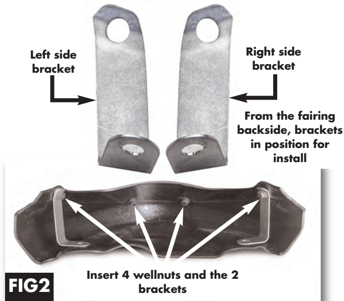
Fig 2. Add wellnuts and brackets provided in there respective place as shown above.
