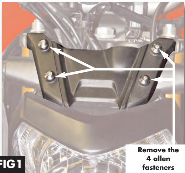
Fig 1. Remove factory allen fasteners as shown above and, set aside for the next step.
