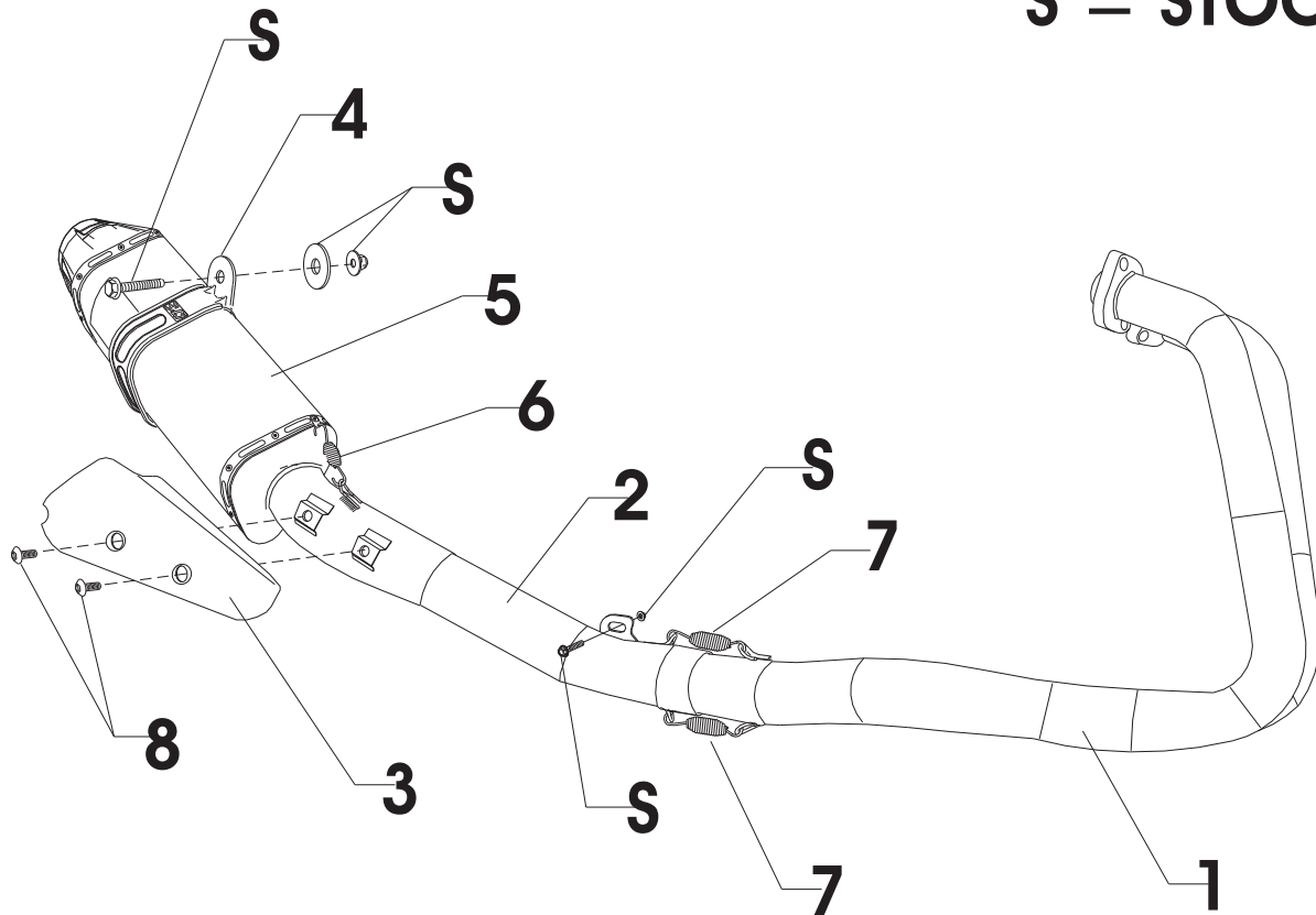
Parts Diagram
