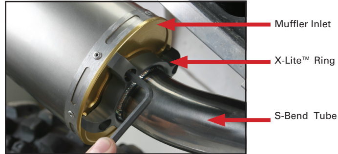
V.A.L.E.™ Assembly Detail
